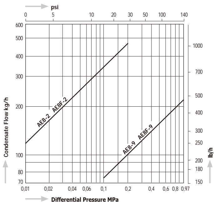
Capacity Chart AE8
