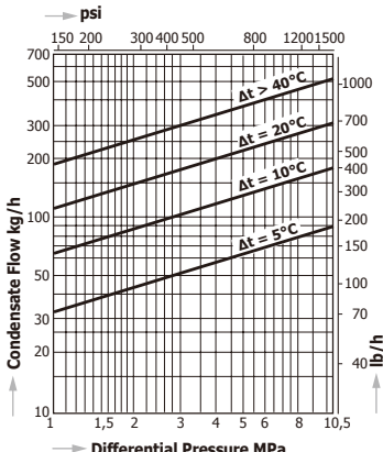
TBH71 - 105
