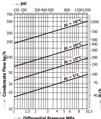
TBH72 - 105
