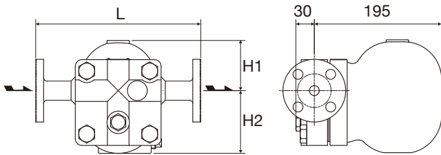
GTH12-F Flanged
