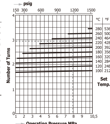
TBH72 - 105
