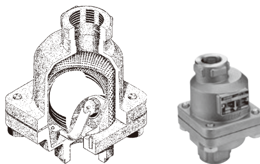
Vertical installation
