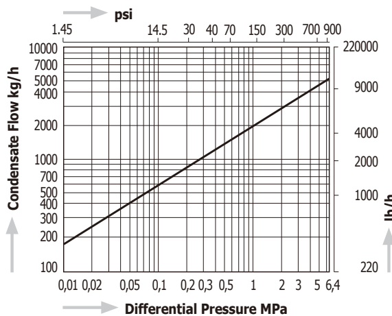
Capacity Chart
